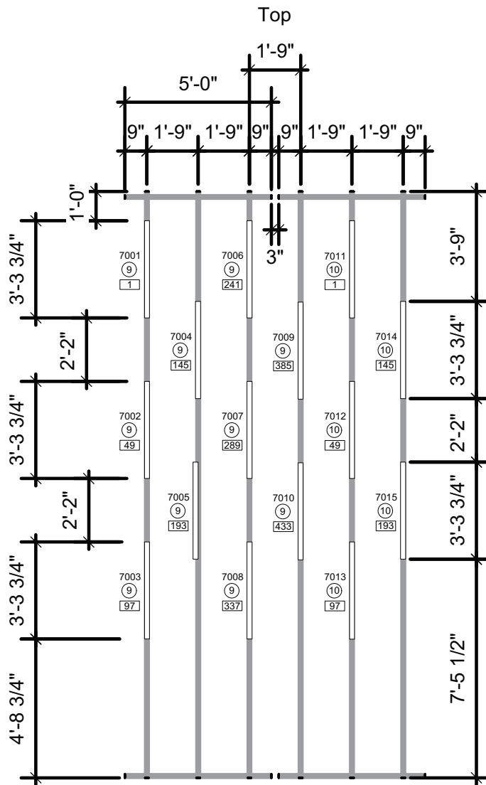
Mega Lite Support Detail
