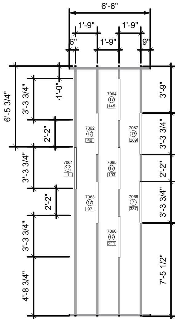
Mega Lite Support Detail End Support
